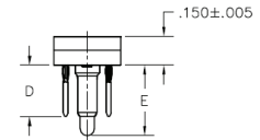
OPTIONAL INSULATOR FOR TOP CONNECTOR WITH TERMINATION OPTIONS: 301, 311, 321, 331, 341, 351, 361, 371 AND 381 (w/CIRCUIT TEST POINT).
